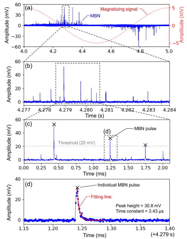
FIGURE 2. (a) Captured MBN pulses from a non-annealed NANOMET ® ribbon. The magnetizing field profile and corresponding MBN signals are shown in red and blue, respectively. (b) A magnified view highlighting individual MBN pulses with the pulse heights exceeding the detection threshold (20 mV). (c) Time-resolved MBN pulse shapes with distinct peak events marked. (d) An example of isolated MBN pulse shown with a fitted decay curve illustrating its steep leading edge and gentle decay profiles, characteristic of DW dynamics.
