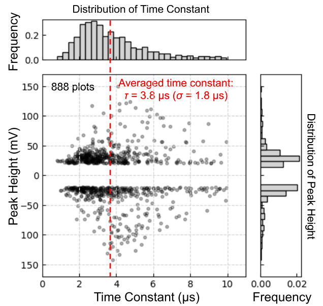
FIGURE 3. Relationship between peak height and time constant obtained from individual MBN pulses at the peak height of 20–170 mV.
