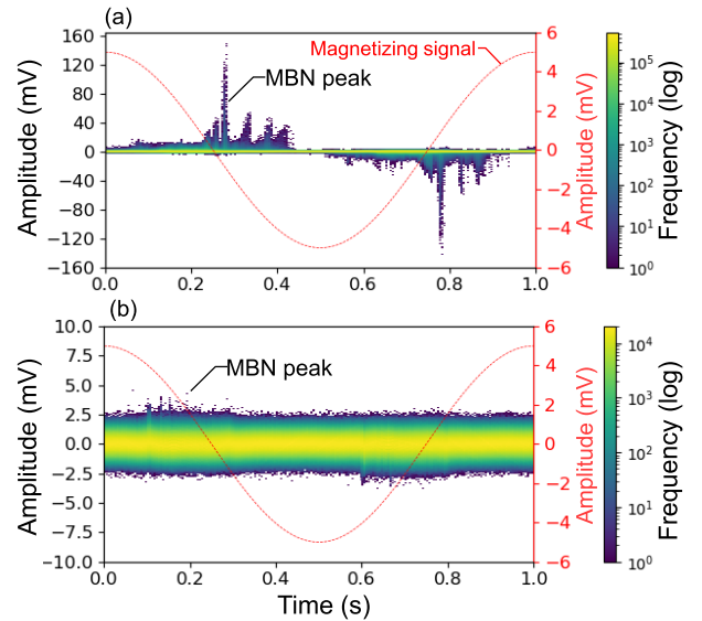
FIGURE 4. Time-resolved frequency distribution of MBN signals for (a) non-annealed and (b) annealed nanocrystalline NANOMET ® ribbons over 100 magnetization cycles.
